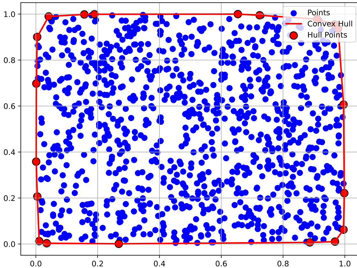
Convex Hull Visualization
