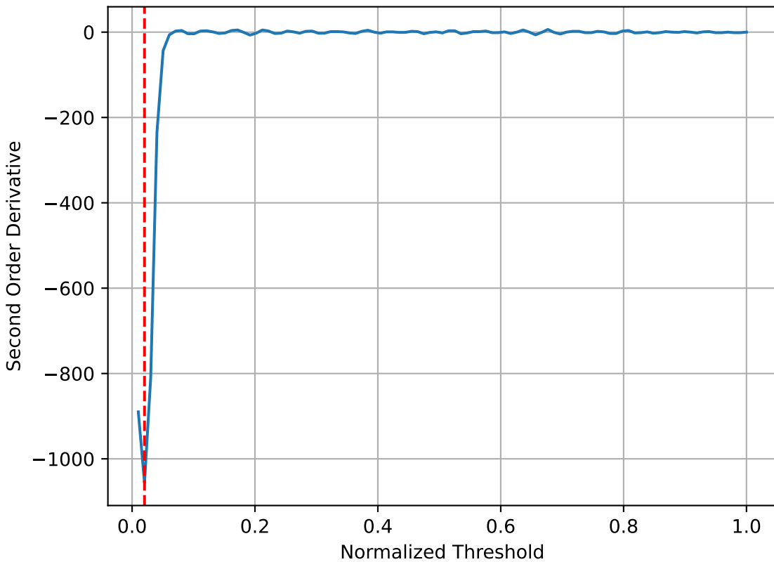
Second Order Derivative Curve
