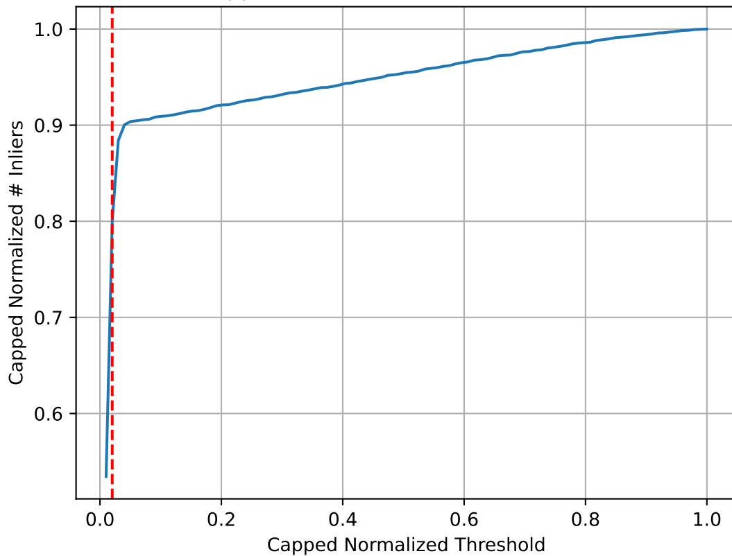
Capped Normalized Inlier Ratio Curve
