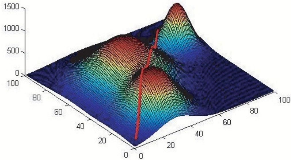
Fig. 2: A 2D world with obstacles depicted as cost functions. Shown in red is a straight line path between two locations. The path has high cost because it passes through/near obstacles.
