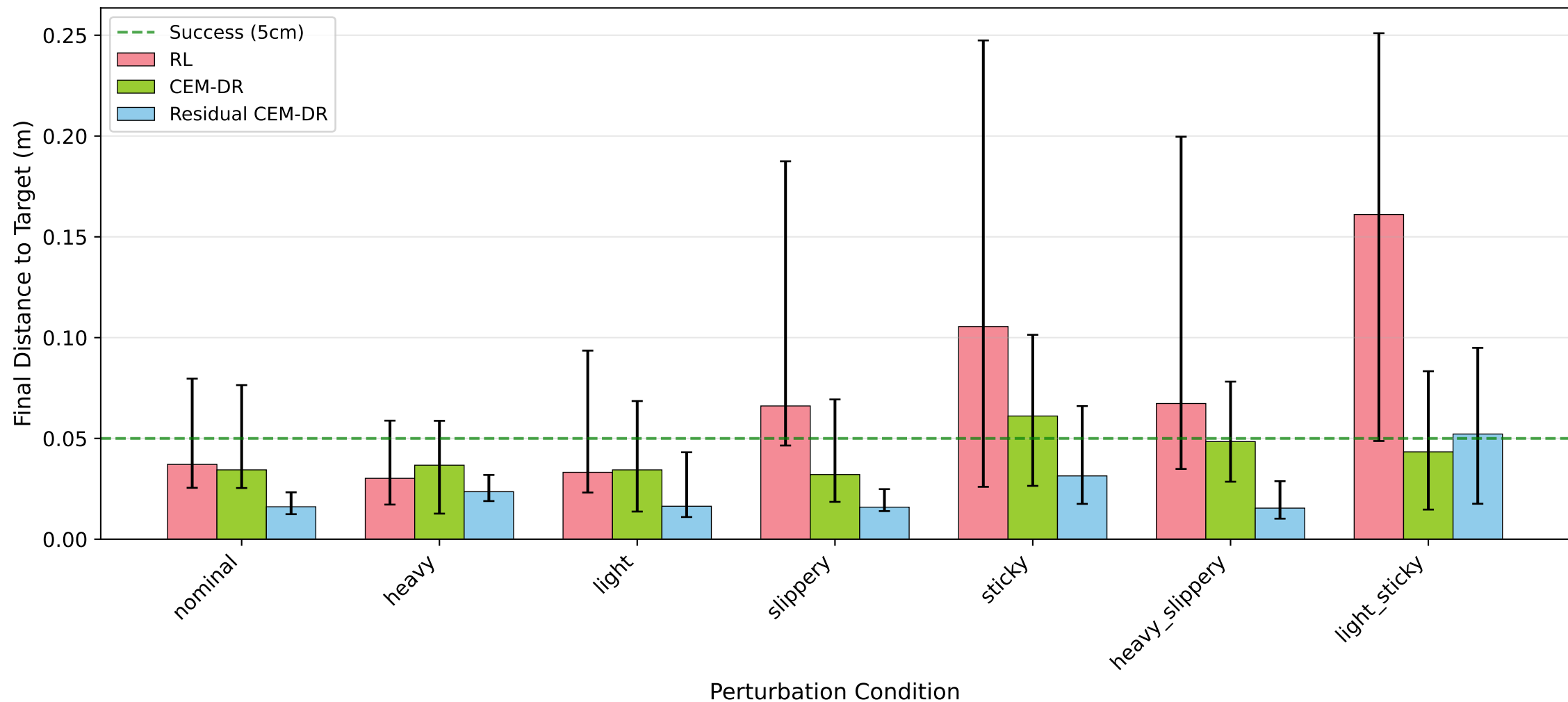
Domain Randomization Experiment: RL vs CEM-DR vs Residual CEM-DR (Median + IQR)
