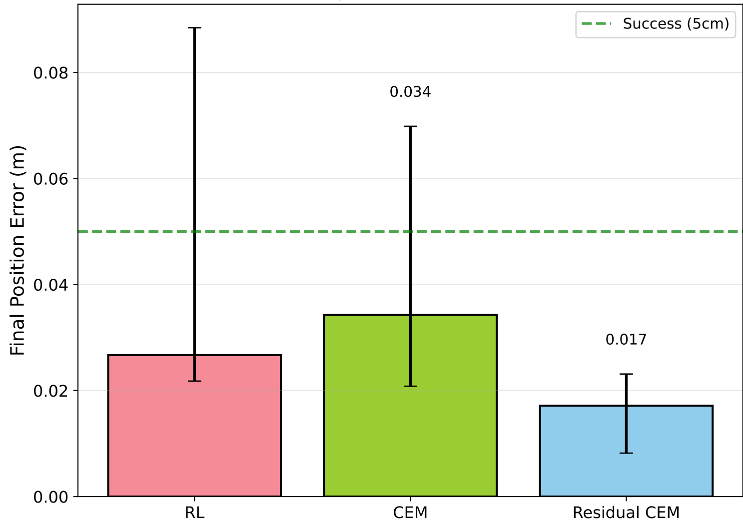
Final Error Comparison - Median + IQR (n=16)
