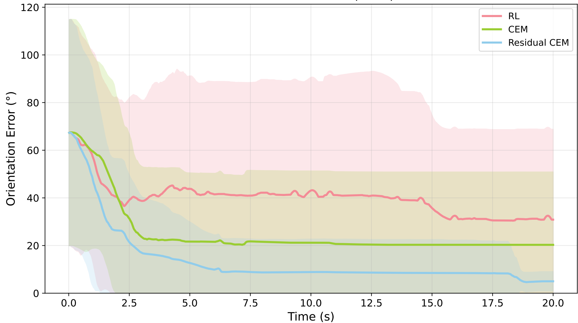
Box Orientation Error (n=16)
