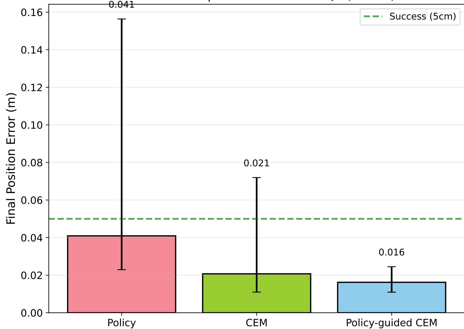
Final Error Comparison - Median + IQR (n=100)
