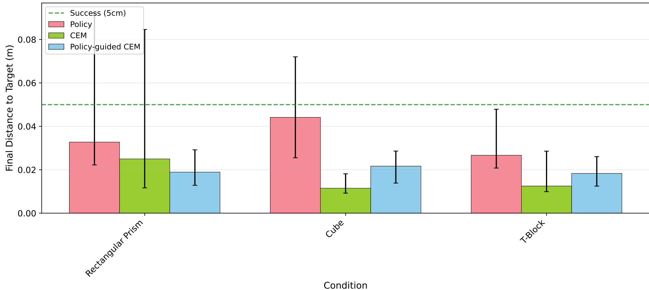
Robustness Comparison: Policy vs CEM vs Policy-guided CEM (Median + IQR)
