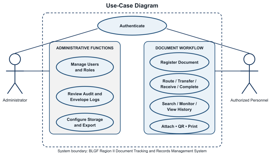
Figure 4. Use-Case Diagram
