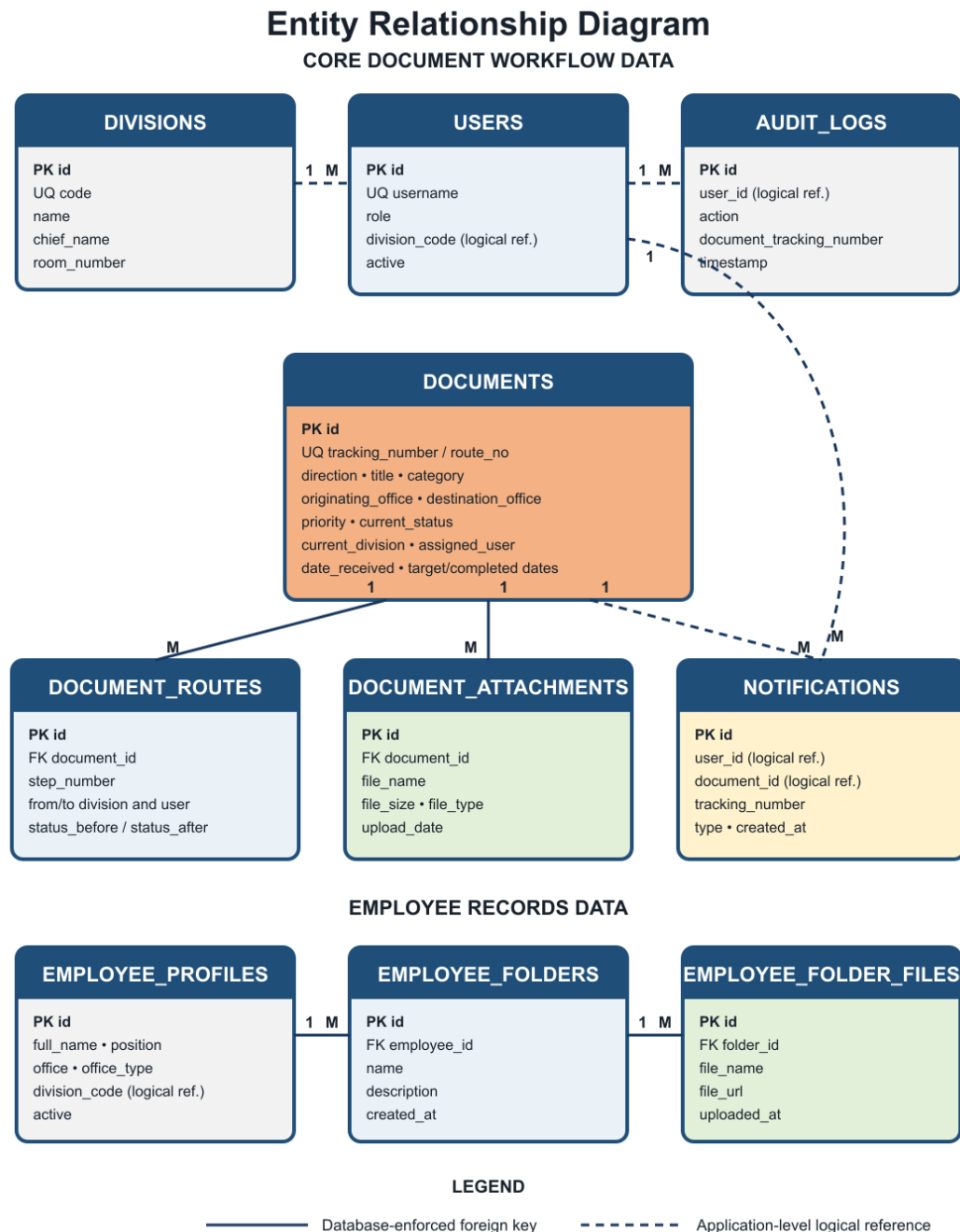
Figure 8. Entity Relationship Diagram
