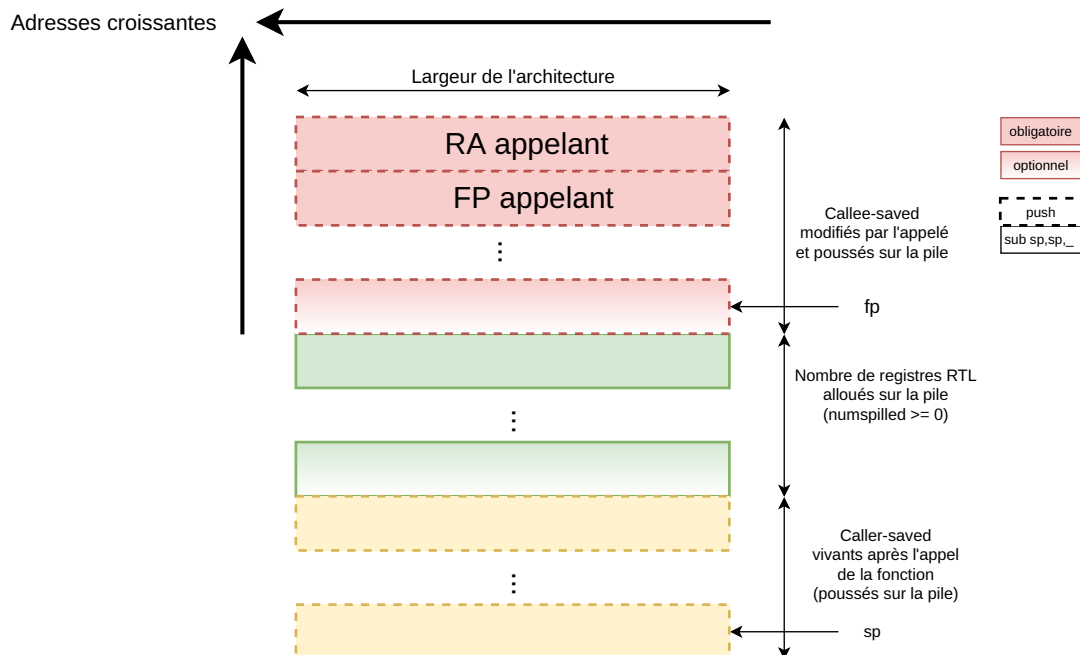
Figure 18: Backup of caller-save registers
