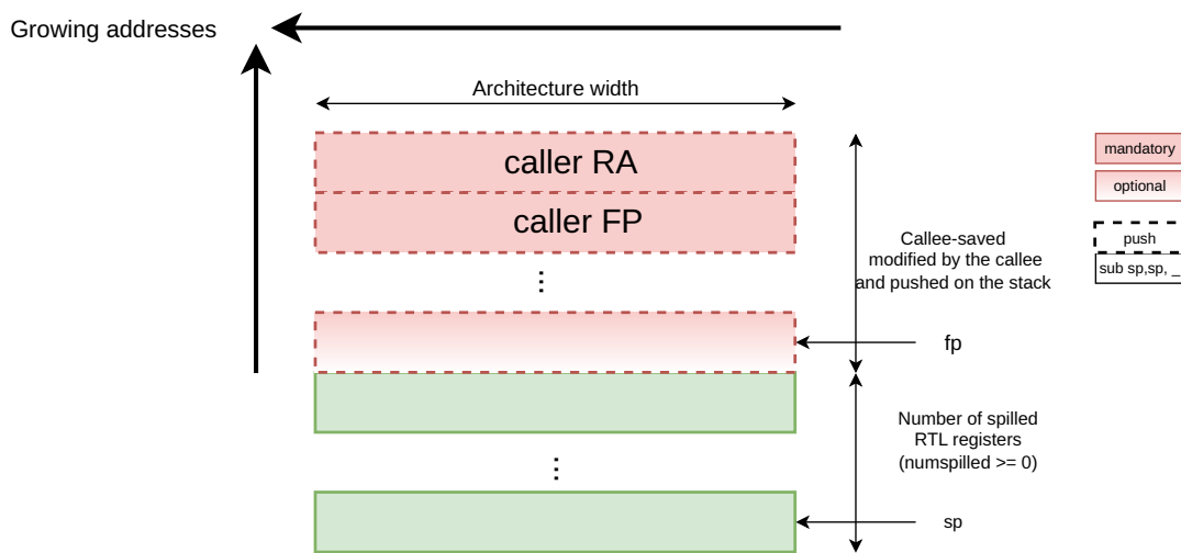
Figure 20: Management of RTL registers allocated on the stack by the register allocator
