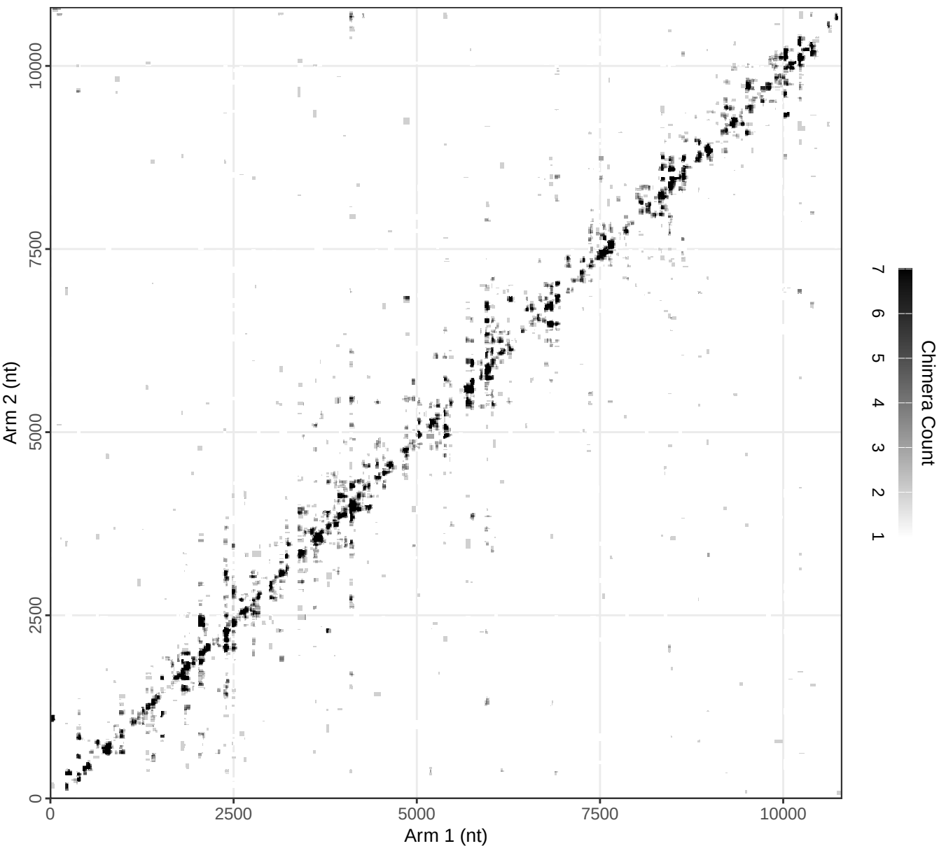
Contact Density Map test.Zika_virusRNA
