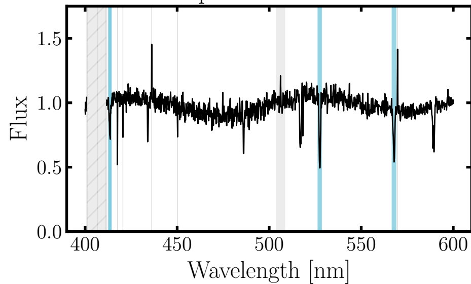
Absorption Line Outlier
