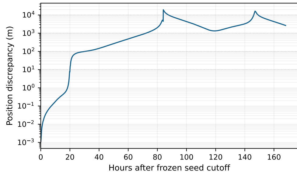
CHANDRA / HEO
