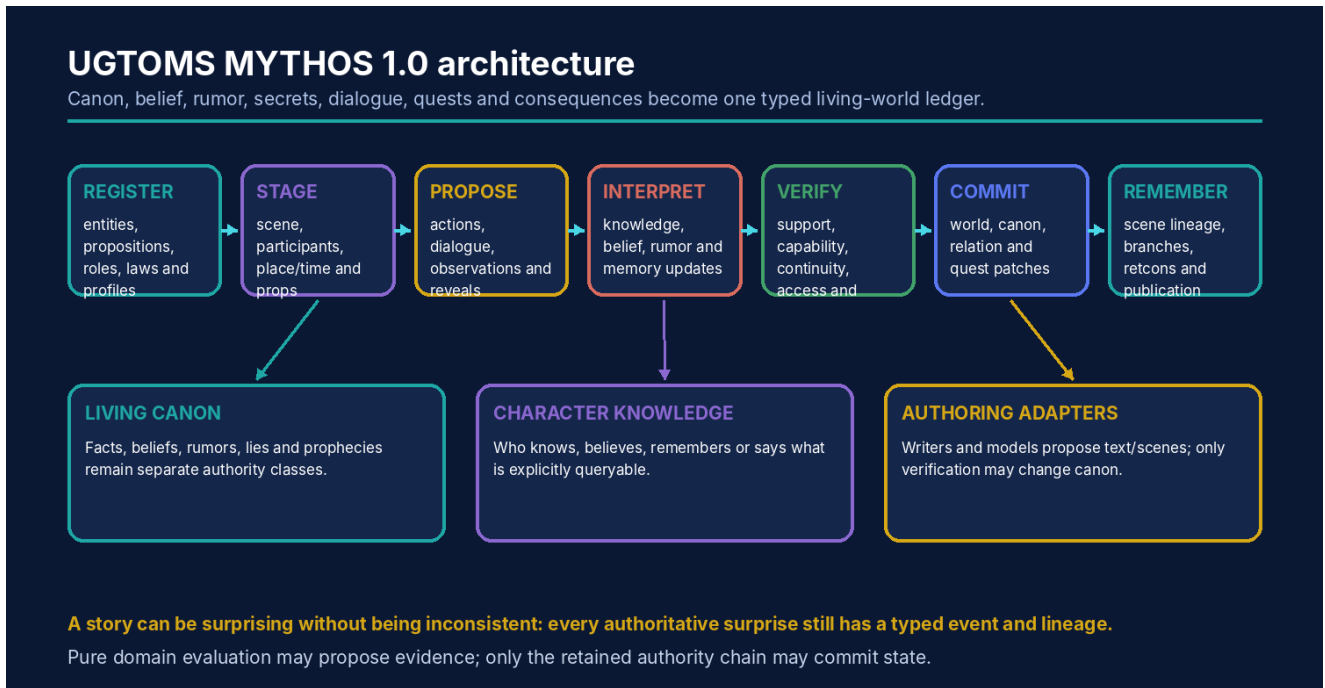
Figure 1. MYTHOS maps narrative authoring and play into the same verified event-authority discipline as other cartridges.
