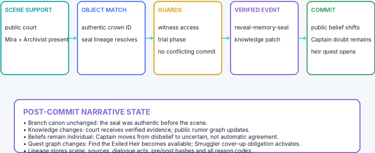
Figure 4. The Crown revelation updates knowledge, relationships and quests while keeping the underlying hidden fact and individual beliefs typed.
