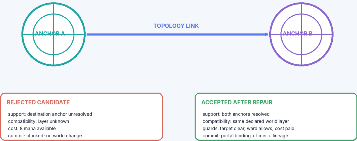
Figure 3. The same spell graph is rejected with an unresolved destination and accepted after typed repair.
