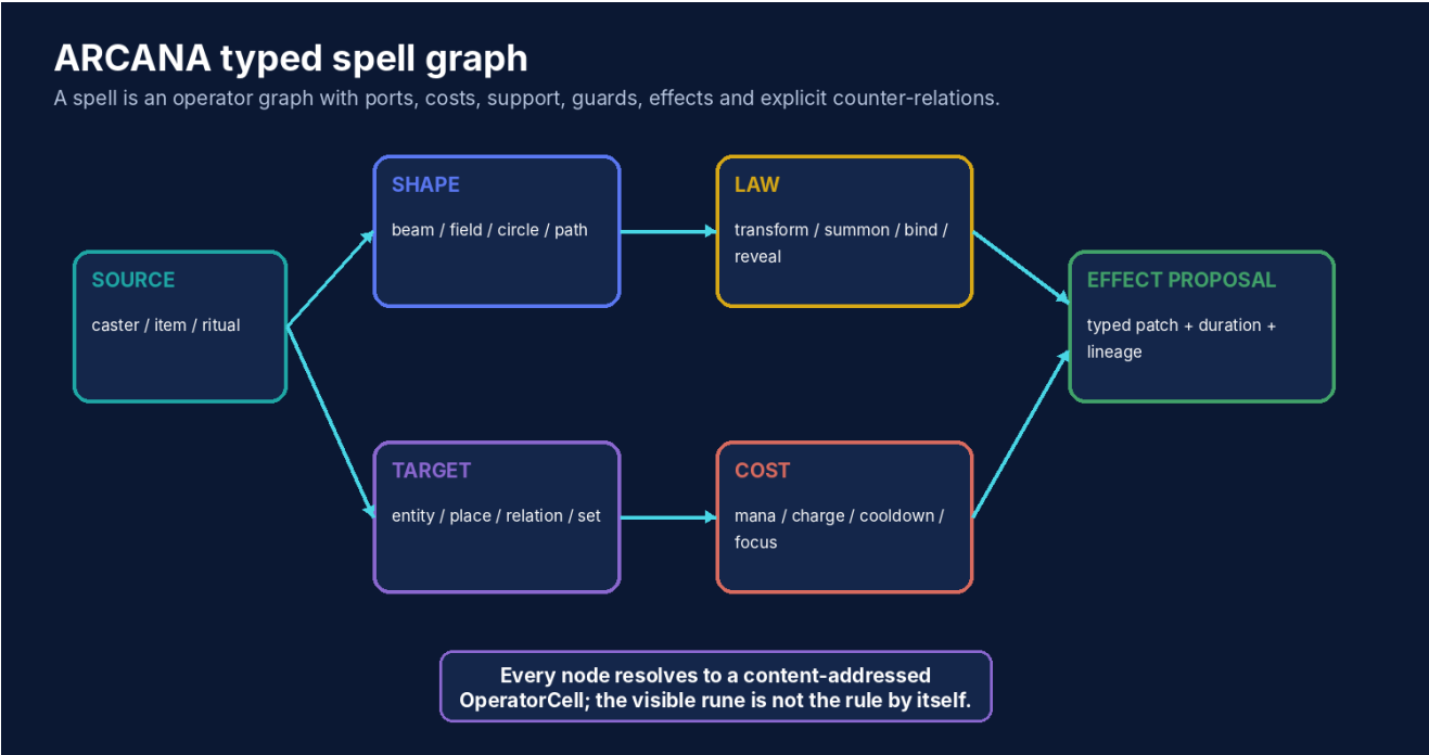
Figure 1. A spell is a typed operator graph; its visible rune is one face of a content-addressed definition.
