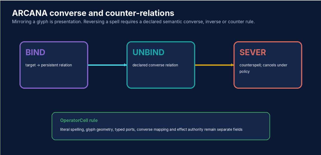
Figure 2. Bind, unbind and sever are distinct declared relations; mirroring the glyph does not choose among them.
