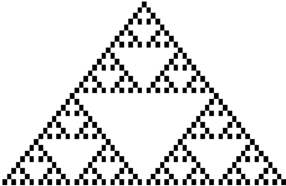
Pascal odd/even parity -> Sierpinski test pattern
