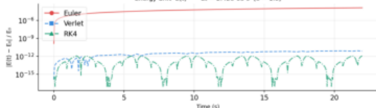
Energy drift E(t) — dt = 2.20e-04 s ( e = 1.0 )
