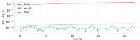
Energy drift E(t) — dt = 1.82e-02 s ( e = 1.0 )
