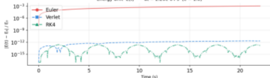
Energy drift E(t) — dt = 2.00e-03 s ( e = 1.0 )
