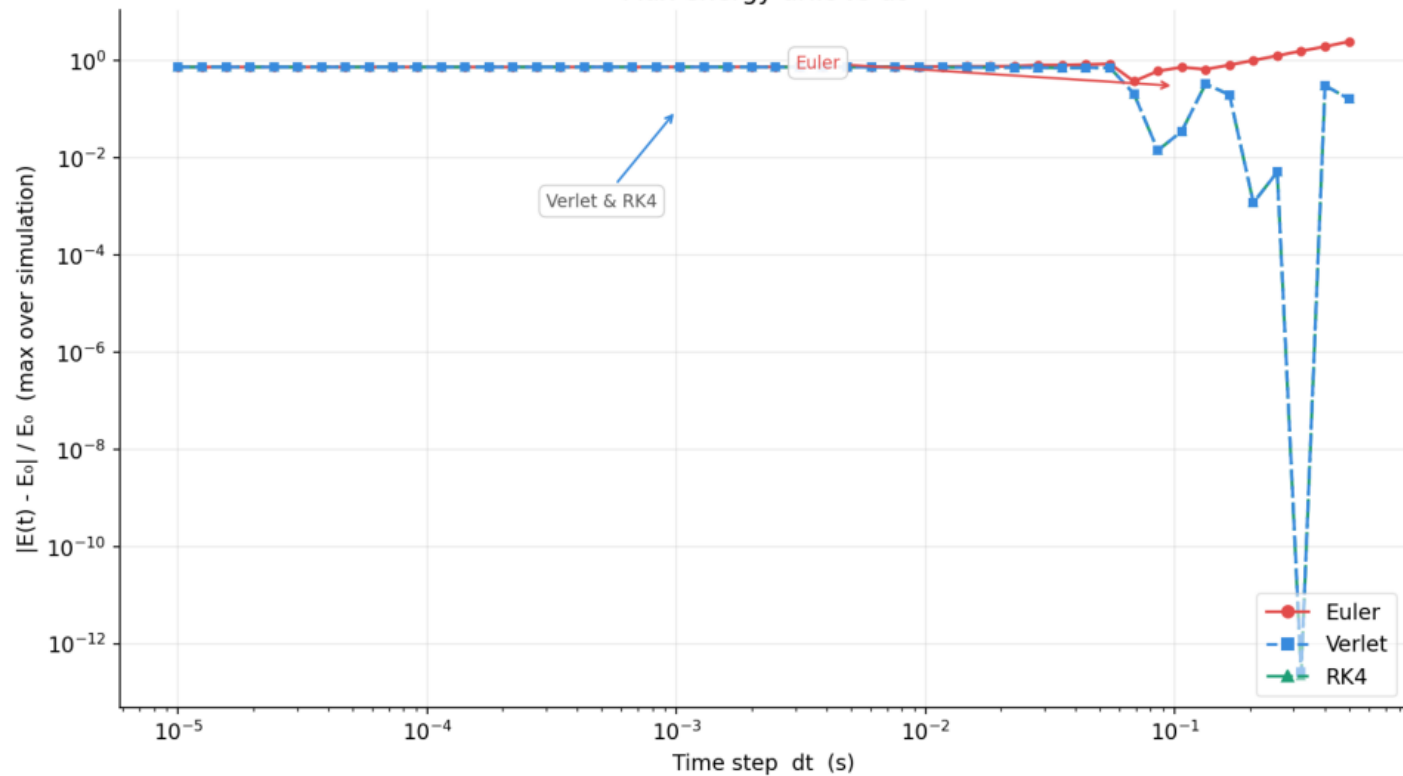
Max energy drift vs dt
