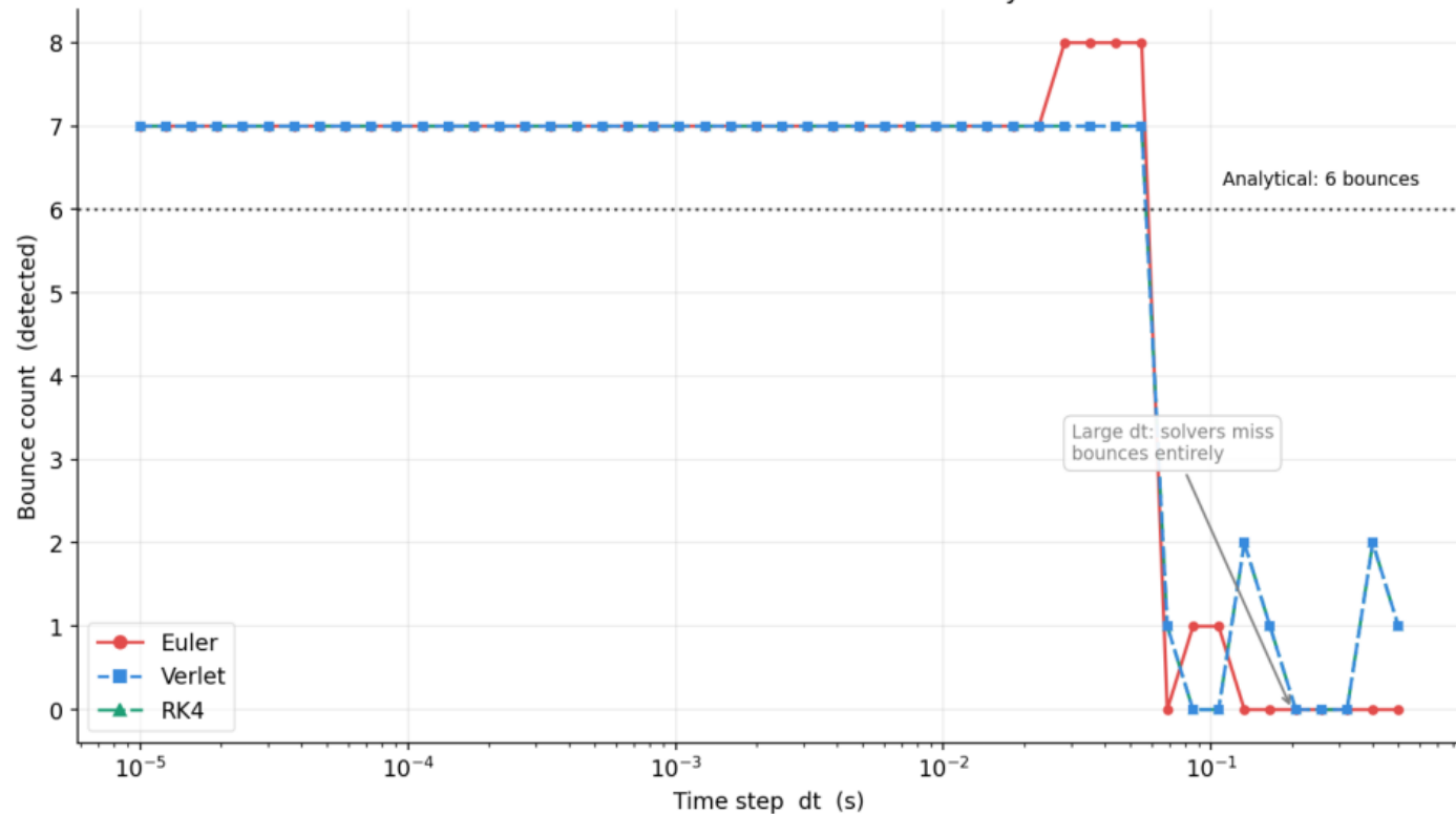
Bounce count vs dt — solver stability
