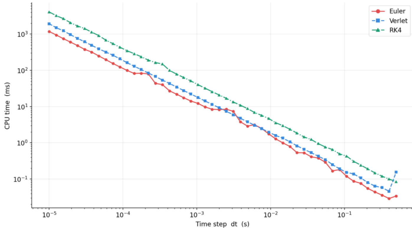
CPU time vs dt
