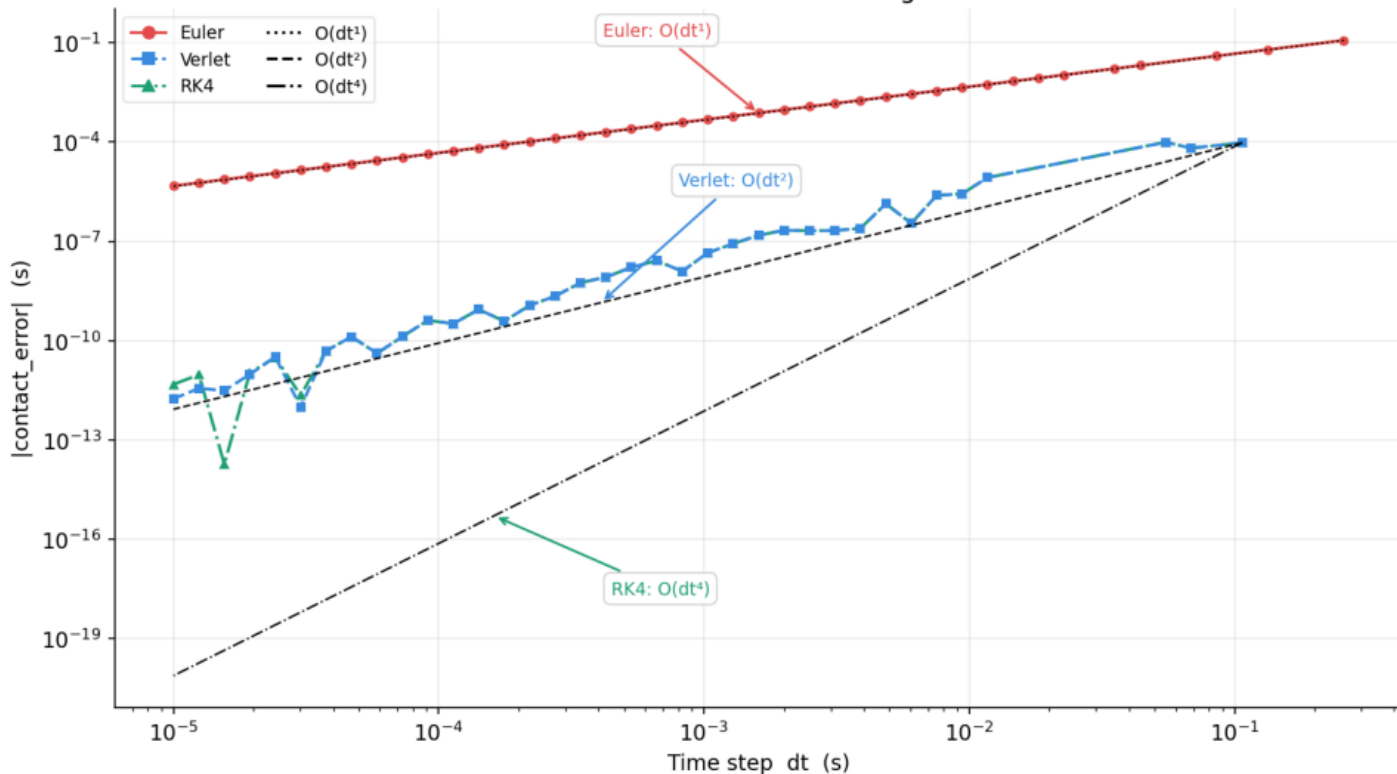
Contact time error vs dt — convergence order
