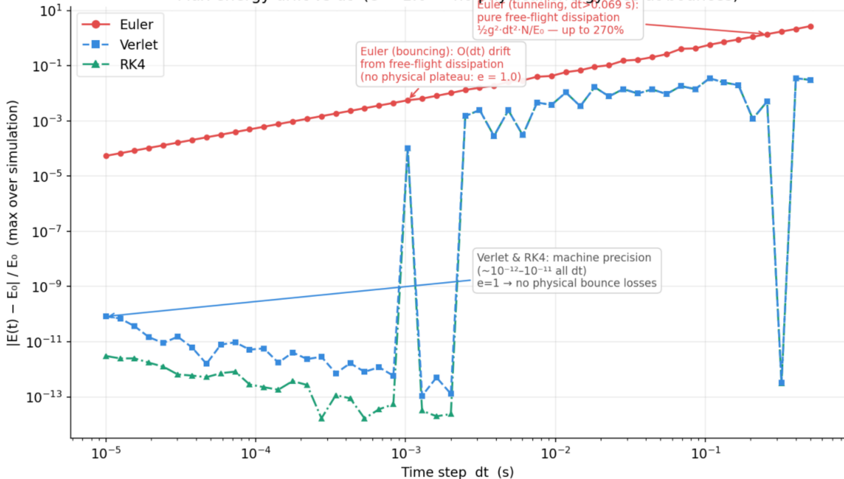
Max energy drift vs dt (e = 1.0 — no physical energy loss at bounces)
