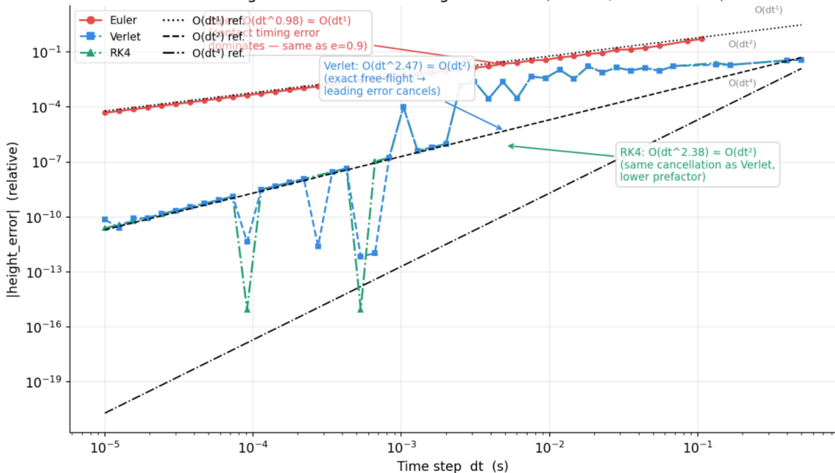
Peak height error vs dt — convergence order (e = 1.0, conservative)
