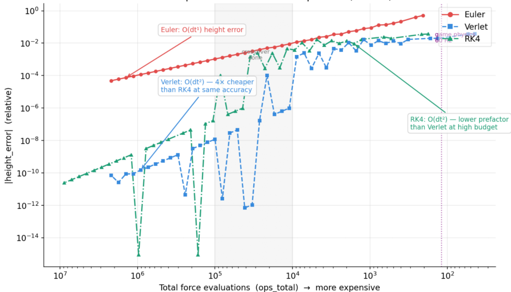
Cost vs precision — iso-cost comparison ( e = 1.0 )
