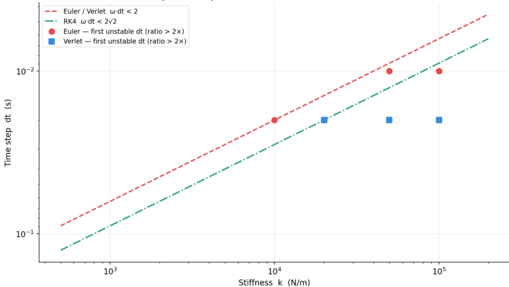
Stability boundary: measured (markers) vs theoretical (lines)
