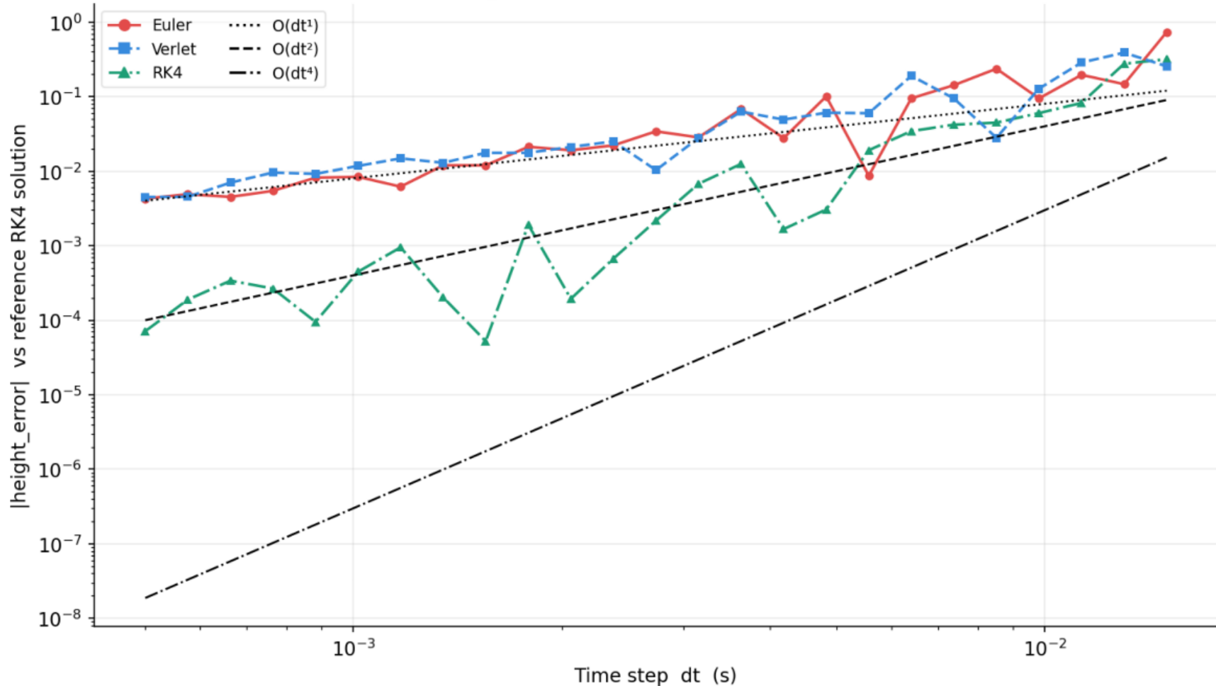
Peak height error vs dt — contact forces mode
