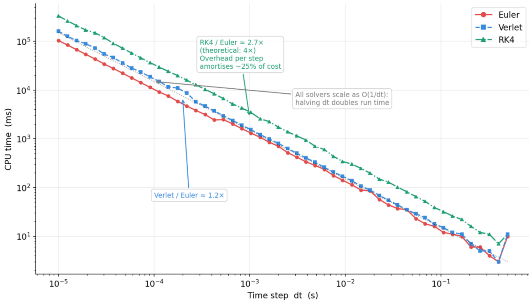
CPU time vs dt
