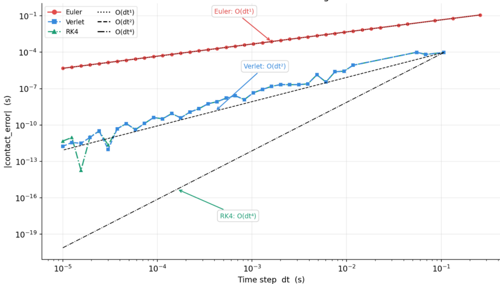
Contact time error vs dt — convergence order
