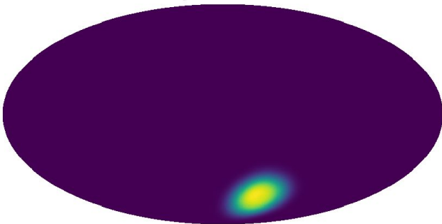
Coverage - Galactic coordinates
