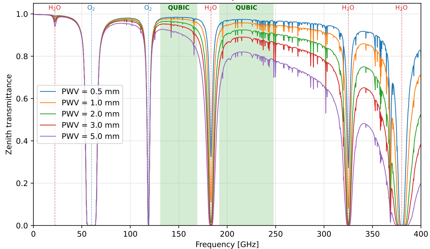
Simulated QUBIC site atmospheric transmittance (am)
