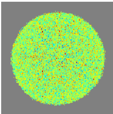
CMB - U - Residual
