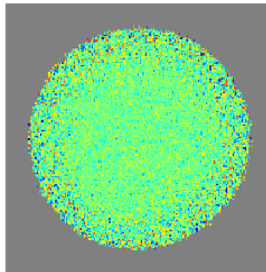
Dust - Q - Residual
