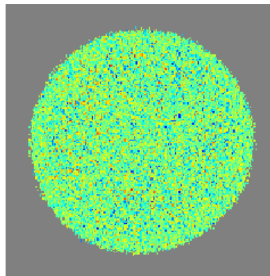
Dust - I - Residual
