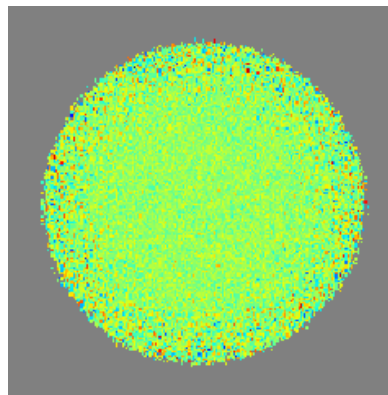
Dust - U - Residual
