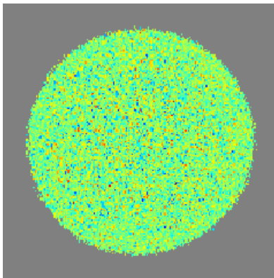
CMB - Q - Residual
