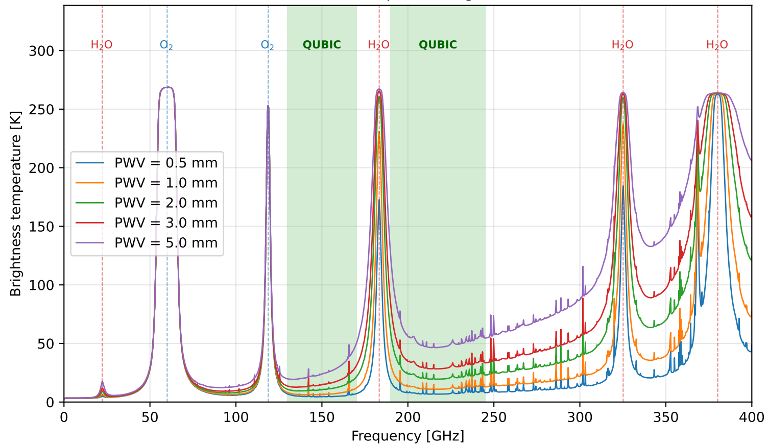
QUBIC site atmospheric brightness (am)
