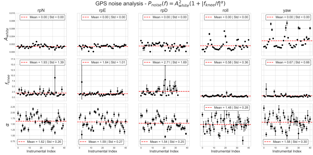
Figure 5.17: Figure to summarize the fitting of the noise model 5.3. The 3 lines represent the three parameters of the model A_{white} , f_{knee} and \alpha . The five columns designate the GPS data. The x-axis is the index of the instrumental configuration, while the y-axis is the value of the model parameter for the given GPS data. In this plot, I removed point with f_{knee} above 10 Hz, as they are not relevant since our sampling rate is 8 Hz.
