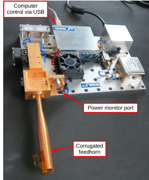
Figure 5.2: Picture of the 150 GHz calibration source system, including its electronics and the waveguide horn. Taken from [8]
