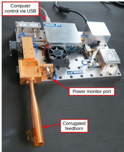
Figure 5.2: Picture of the 150 GHz calibration source system, including its electronics and the waveguide horn. Taken from [17]
