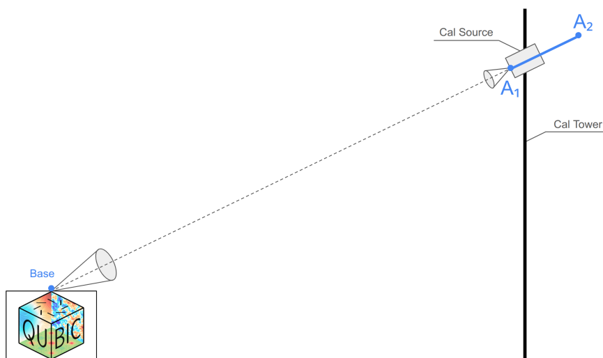
Figure 1.20: Drawing to show the expected position for the GPS antennas. The base antenna is located as close as possible from QUBIC line-of-sight, on the left. On the right, the Calibration Source is fixed on the Calibration Tower, the Antenna 1 (A1) is attached as close as possible from the line-of-sight of the source, while the Antenna 2 (A2) is placed on a rigid rod, again align with the line-of-sight.
