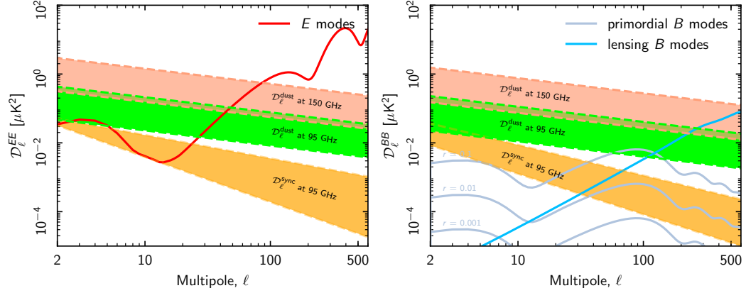
Figure 1.21: (left) Dust (95 and 150 GHz) and synchrotron (95 GHz) E-modes power versus CMB. (right) Dust (95 and 150 GHz) and synchrotron (95 GHz) B-modes power versus CMB ( r = 0.1, 0.01, 0.001 ). The coloured bands show the range of power measured from the smallest to the largest sky regions in Planck analysis. Taken from [50].
