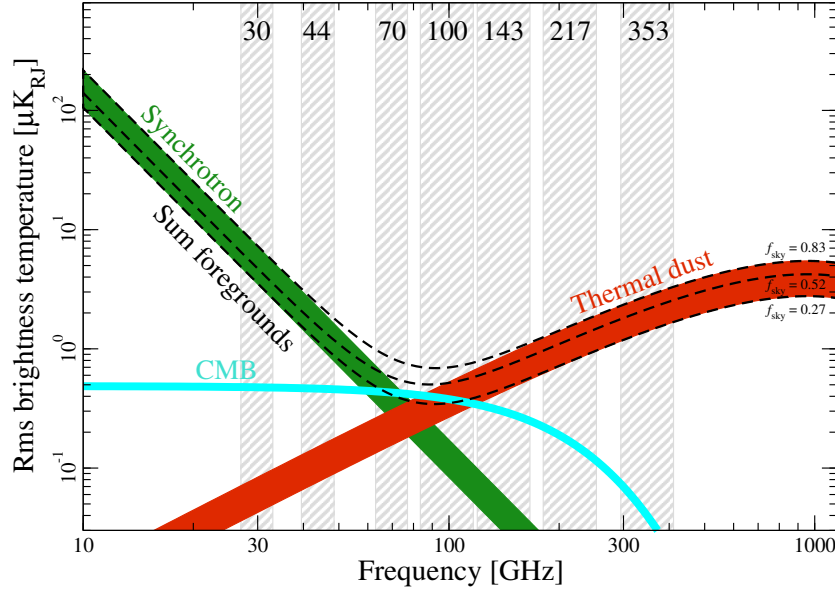
Figure 1.20: Planck’s measurements of polarization amplitude rms as a function of frequency for polarised synchrotron emission (green), polarised thermal dust emission (red) and CMB polarisation (cyan). The dashed black lines indicate the sum of foregrounds evaluated over three different masks with f_{\text{sky}} = 0.83 , 0.52 , and 0.27 . The widths of the synchrotron and thermal dust bands are defined by the largest and smallest sky coverages. Taken from [52].
