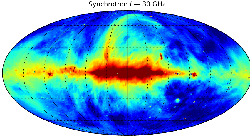
Figure 1.18: Synchrotron intensity map at 30 GHz from the Planck Commander analysis [52].
