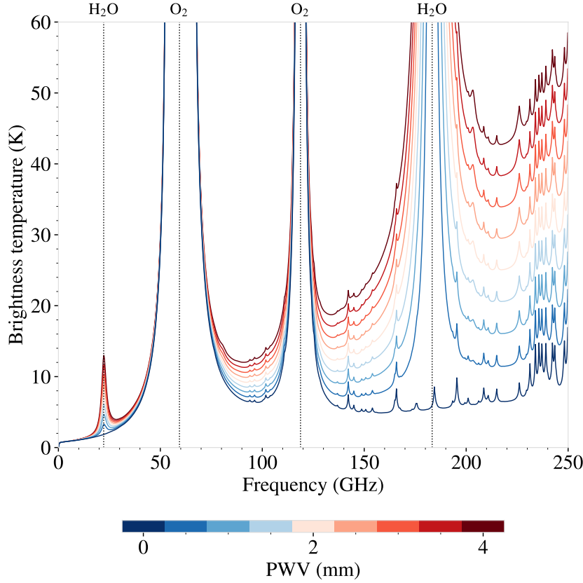
Figure 1.22: One-year average zenith atmospheric brightness for different values of Precipitable Water Vapour (PWV). The main H_2O and O_2 absorption lines are indicated. Taken from [53].
