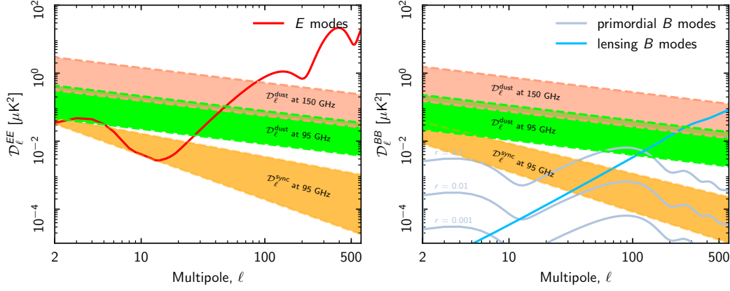
Figure 1.17: (left) Dust (95 and 150 GHz) and synchrotron (95 GHz) E-modes power versus CMB. (right) Dust (95 and 150 GHz) and synchrotron (95 GHz) B-modes power versus CMB ( r = 0.1, 0.01, 0.001 ). The coloured bands show the range of power measured from the smallest to the largest sky regions in Planck analysis. Taken from [50].
