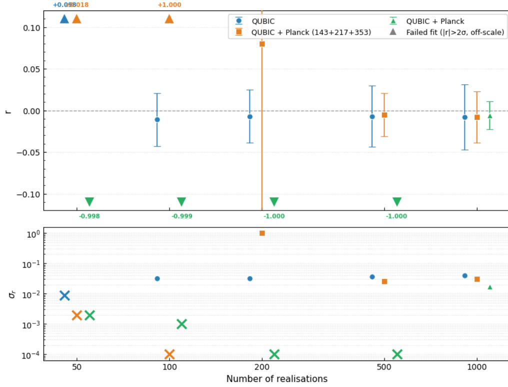
Figure 1.7: Recovered tensor-to-scalar ratio r (top) and corresponding uncertainty \sigma_r (bottom) as a function of the number of noise realisations used in the debiasing procedure. The three colours correspond to different sets of frequency channels included in the fit. Triangles and crosses indicate configurations for which the recovered value of r is not statistically compatible with the input value r = 0 .
