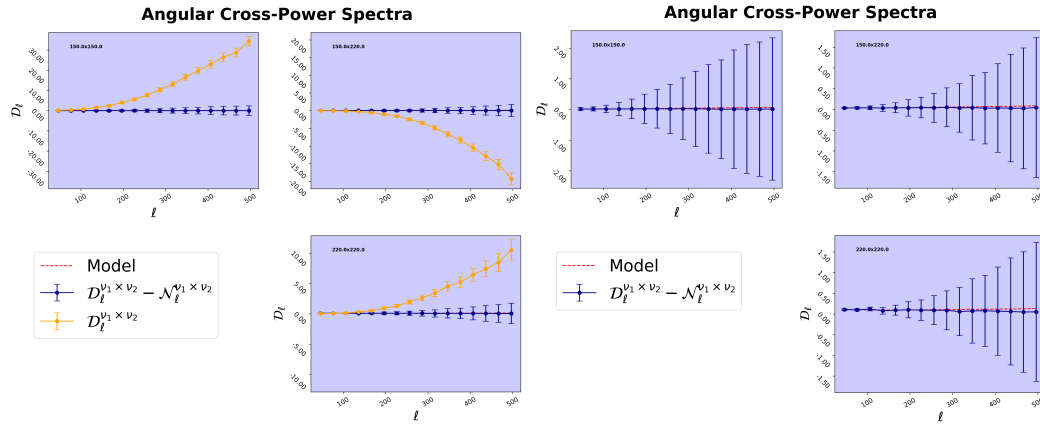
Figure 1.1: Comparison between biased and unbiased cross-power spectra computed over two frequency maps. (left) The orange points are spectra containing sky signal and noise, while blue points are the spectra where we removed the noise bias. Red dash line shows the theoretical model for the signal spectra. (right) Same figure without the biased spectra, to show that the result are indeed centered around the model.
