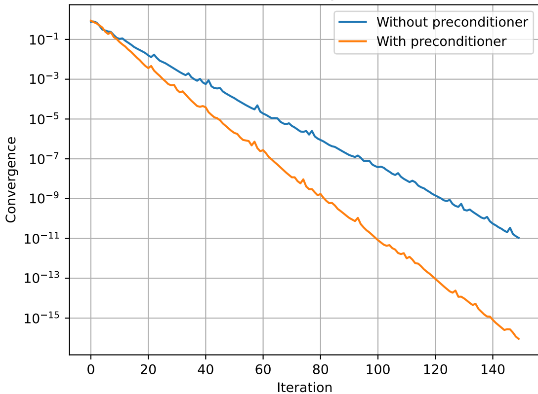
PCG Convergence
