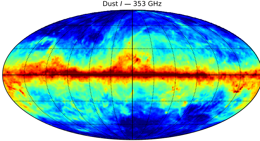
Figure 1.17: Thermal dust intensity map at 353 GHz from the Planck Commander analysis [64].
