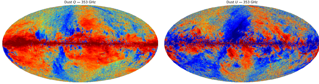
Figure 1.18: Thermal dust polarisation maps at 353 GHz from the Planck Commander analysis [64]. (left) Stokes Q map. (right) Stokes U map.
