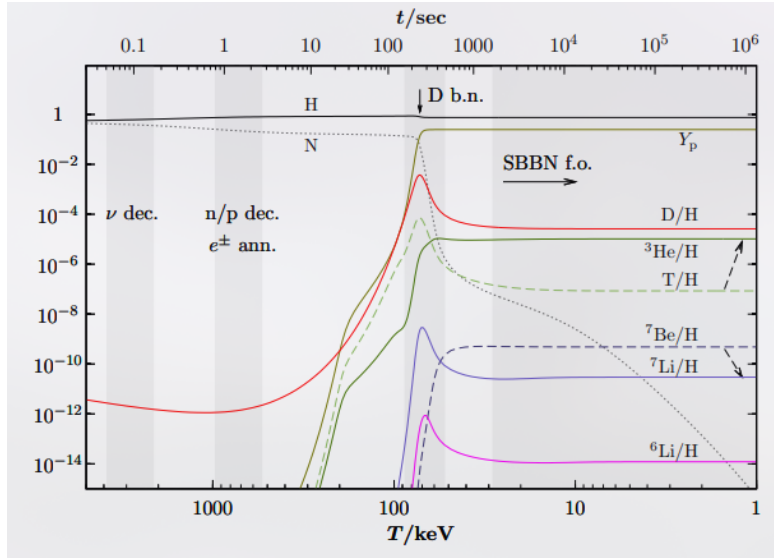
Figure 1.6: Illustration of the Big Bang Nucleosynthesis process, showing the abundances of elements with time (top-axis) and energy (bottom-axis). Taken from [40].
