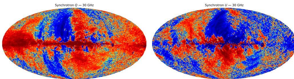
Figure 1.20: Synchrotron polarisation maps at 30 GHz from the Planck Commander analysis [64]. (left) Stokes Q map. (right) Stokes U map.
