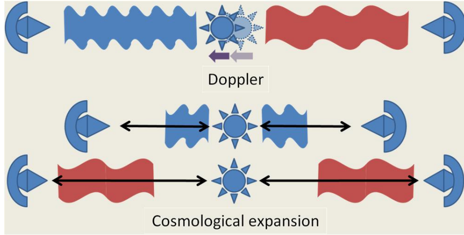
Figure 1.2: Illustration, from [8], showing the difference between Doppler redshift and cosmological redshift. Doppler’s redshift [6], on top, is the decrease in wavelength of an object approaching us, and the broadening of an object moving away from us. Cosmological’s redshift [3] is the broadening of the wavelength in all directions due to the expansion of the Universe.
