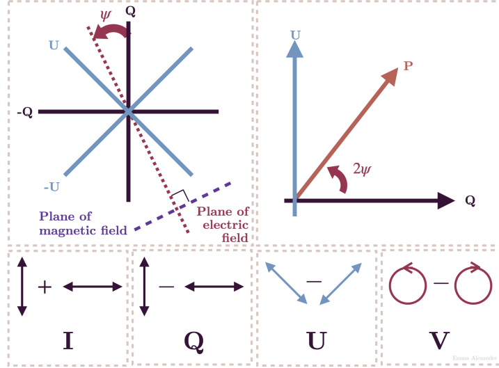
Figure 1.13: Visual representation of the Stokes parameters. Image from Wikimedia Commons [56].
