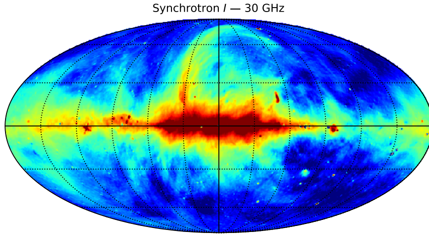
Figure 1.19: Synchrotron intensity map at 30 GHz from the Planck Commander analysis [64].
