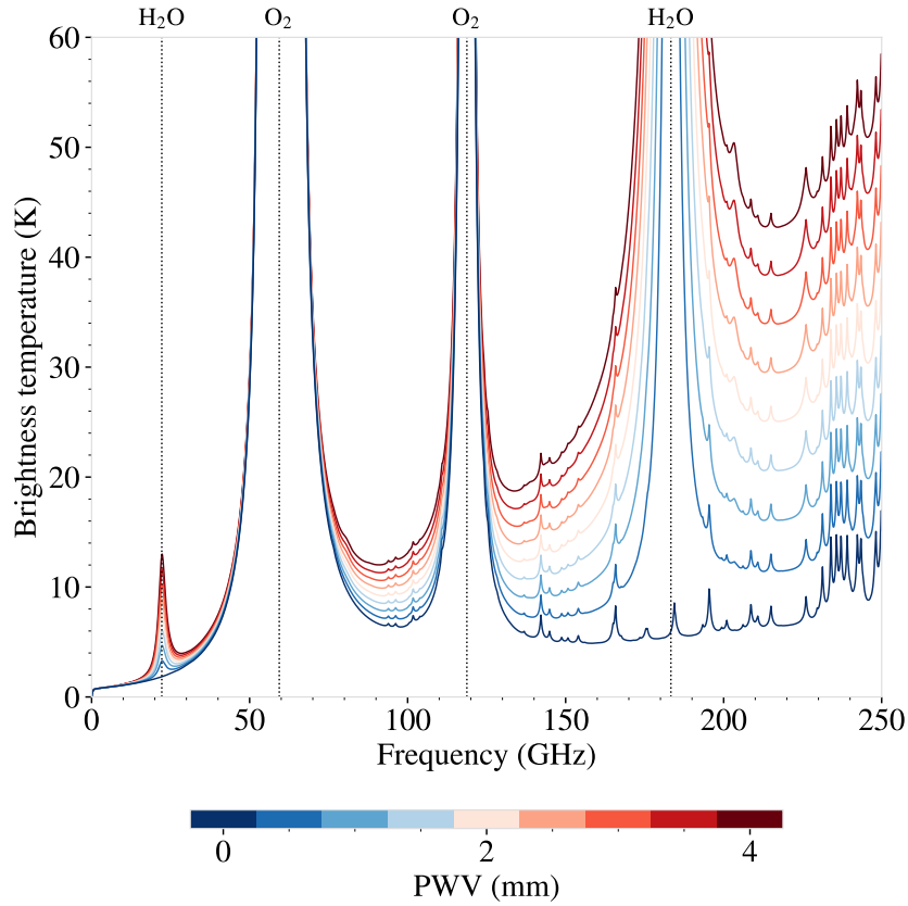
Figure 1.23: One-year average zenith atmospheric brightness for different values of Precipitable Water Vapour (PWV). The main H_2O and O_2 absorption lines are indicated. Taken from [65].
