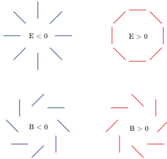
Figure 1.14: Visual representation of the E and B modes. Image from Wikimedia Commons [57].
