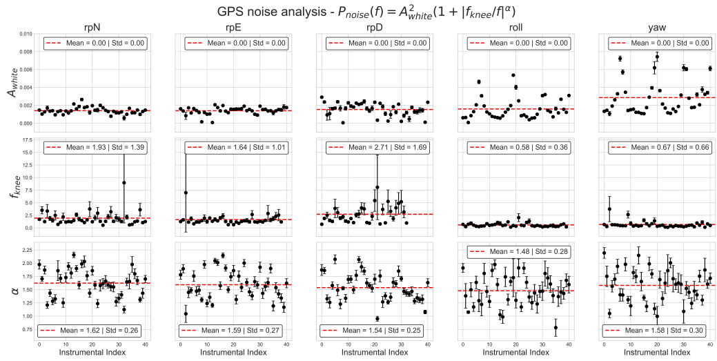
Figure 1.17: Figure to summarize the fitting of the noise model 1.3. The 3 lines represent the three parameters of the model A_{white} , f_{knee} and \alpha . The five columns designate the GPS data. The x-axis is the index of the instrumental configuration, while the y-axis is the value of the model parameter for the given GPS data. In this plot, I removed point with f_{knee} above 10 Hz, as they are not relevant since our sampling rate is 8 Hz.
