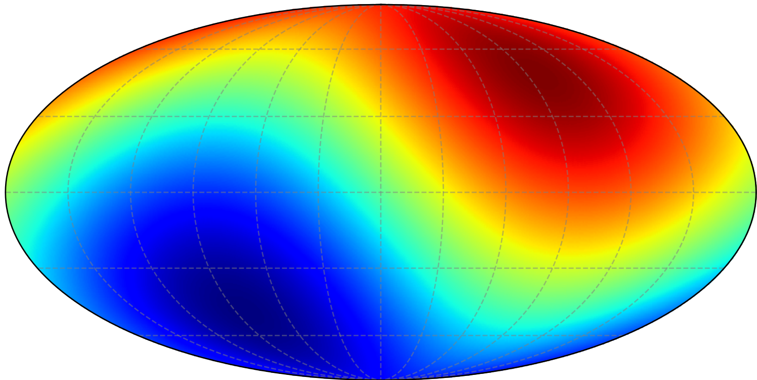
CMB Solar Dipole
