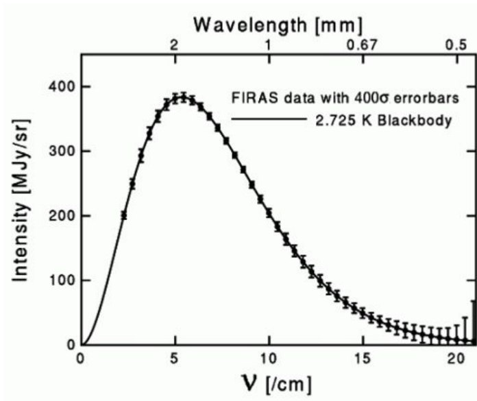
Figure 1.8: CMB spectrum measured by FIRAS instrument on COBE satellite. Plain line is the theoretical spectrum for a blackbody at 2.725 K, points are data from FIRAS with error bars multiplied by 400 to be visible.
