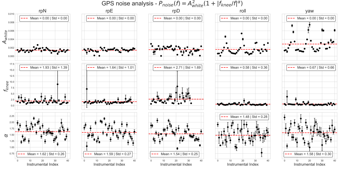
Figure 1.17: Figure to summarise the fitting of the noise model 1.3. The 3 lines represent the three parameters of the model A_{white} , f_{knee} and \alpha . The five columns designate the GPS data. The x-axis is the index of the instrumental configuration, while the y-axis is the value of the model parameter for the given GPS data. In this plot, I removed point with f_{knee} above 10 Hz, as they are not relevant since our sampling rate is 8 Hz.
