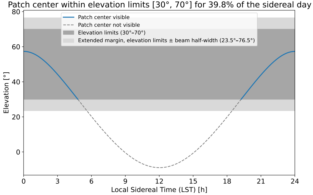
Figure 1.4: Plot showing the visible time of the targeted QUBIC patch during one sidereal day from the instrument point of view. This plot includes the instrumental limitation of observing between [30, 70]^\circ to keep the maximal efficiency of the cryogenic system. In addition, we added the width of the QUBIC beam ( \sim 13^\circ ) in order to compute the maximum time of visibility of the patch.
