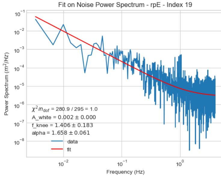
Figure 1.16: Power Spectrum (in blue) for rpE data for the configuration 19. The fitted model 1.3 is displayed (in red) above the data. The parameters value of the model and their associated error is shown, in addition to the \chi^2 value divided by the degree of freedom.
