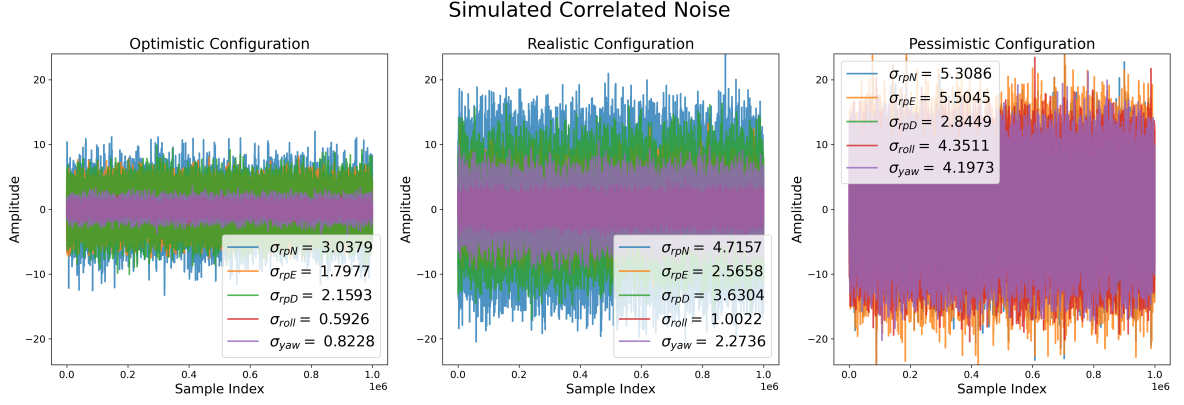
(a) Example of simulated GPS data with correlated noise, for the optimistic, the realistic and the pessimistic configurations. The amplitude of the noise is in millimetres for the position data and in 10^{-3} degrees for the angles. This noise is simulated over one million time samples, with a sampling rate of 8 Hz, same as the real GPS.
