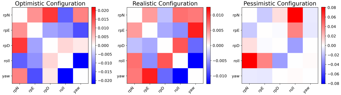
Figure 1.24: Difference element-by-element between the correlation matrix computed from real data and the one computed from simulated data for the three configurations.
