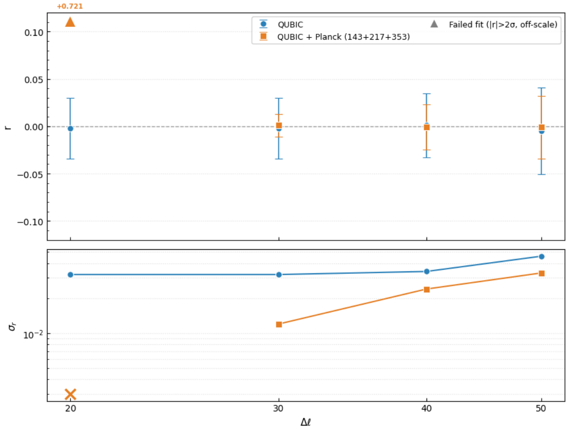
Figure 1.13: Top: fitted value of the tensor-to-scalar ratio r as a function of \Delta_\ell . Error bars correspond to the MCMC uncertainty \sigma_r . Bottom: evolution of \sigma_r as a function of \Delta_\ell .
