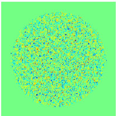
CMB - I - Residual
