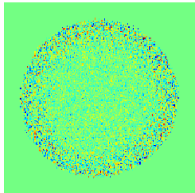
Dust - Q - Residual
