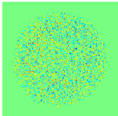
Dust - I - Residual
