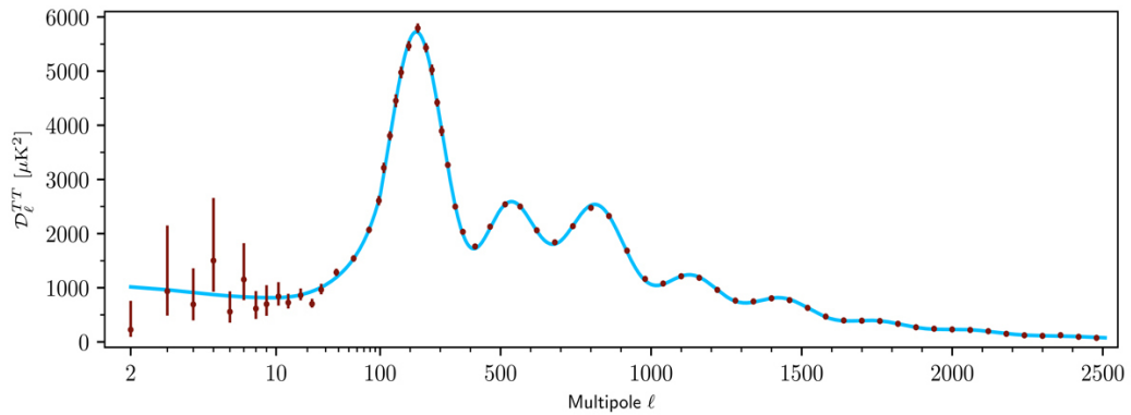
Figure 1.12: Angular power spectrum from Planck Temperature maps. Taken from [41].
