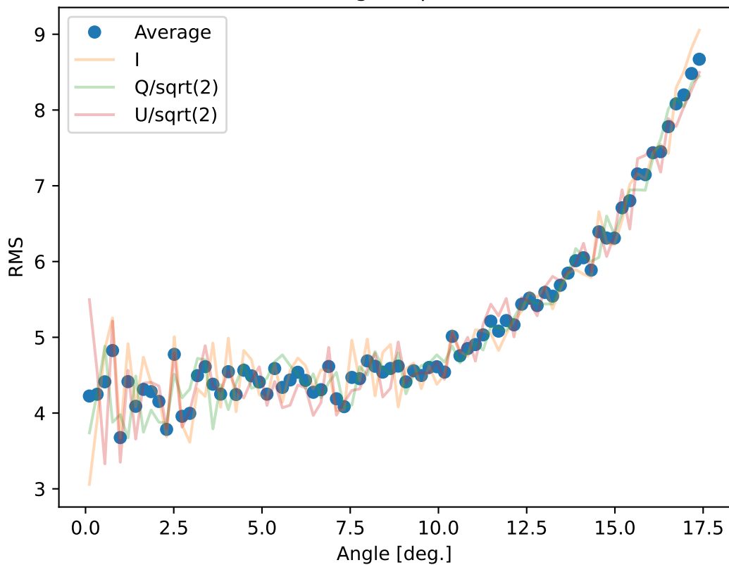
Residual noise angular profile - 140.0 GHz
