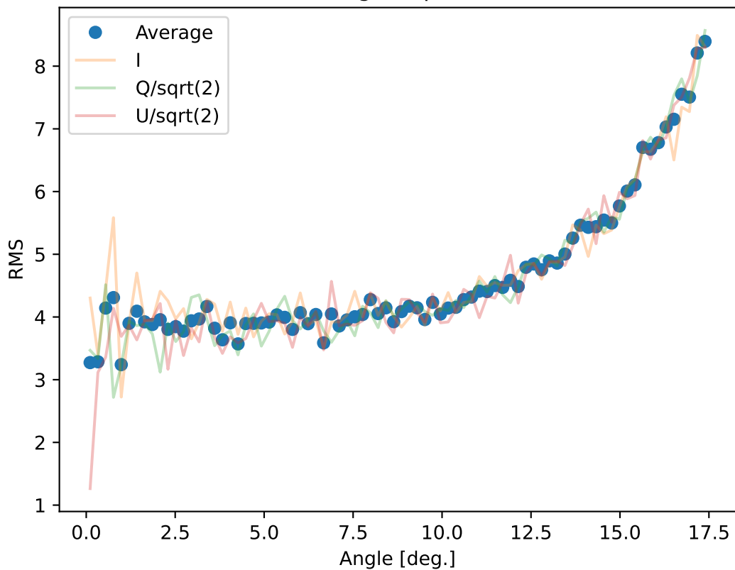
Residual noise angular profile - 159.0 GHz
