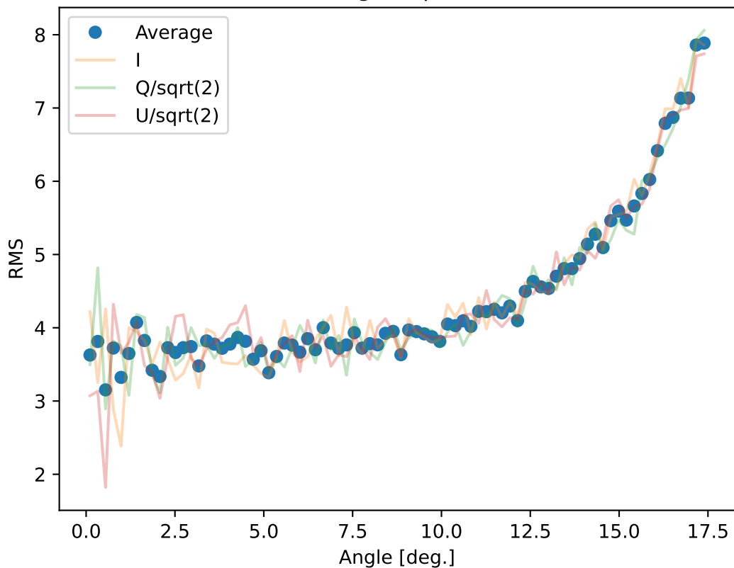
Residual noise angular profile - 205.0 GHz
