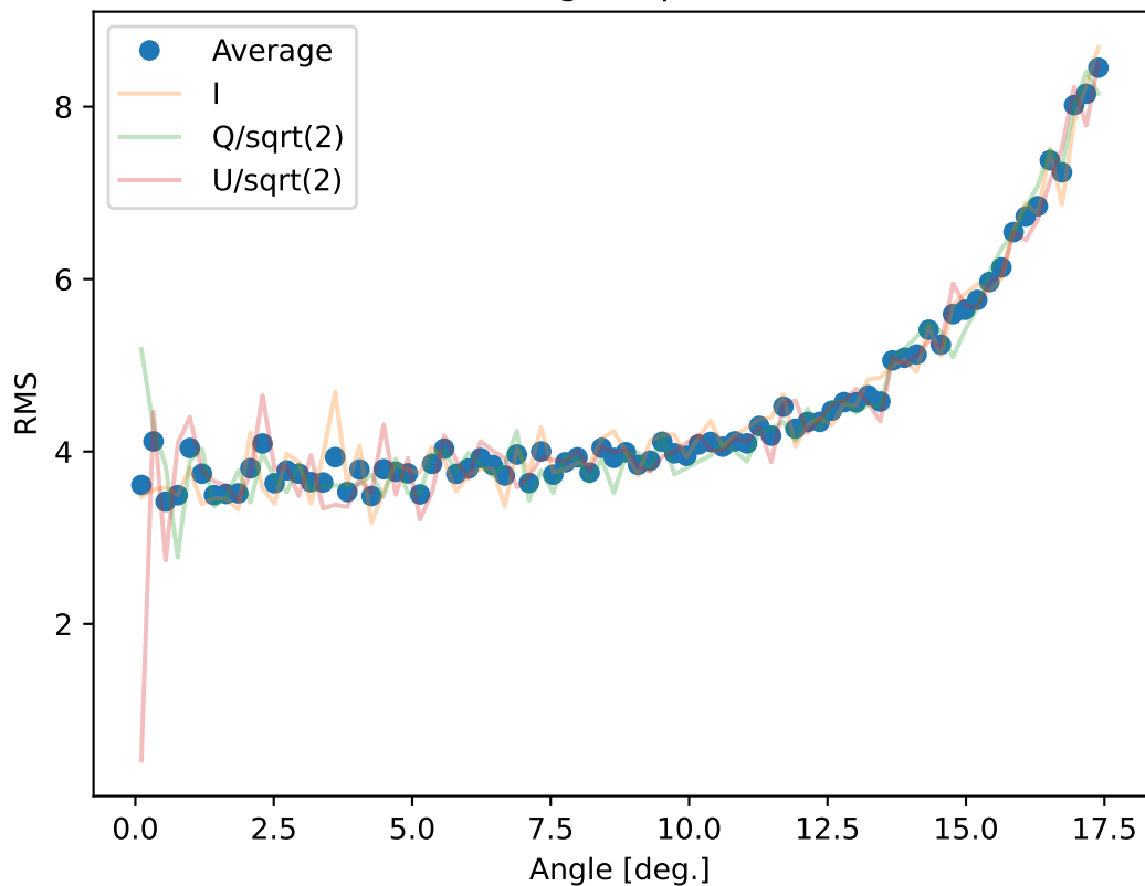
Residual noise angular profile - 233.0 GHz
