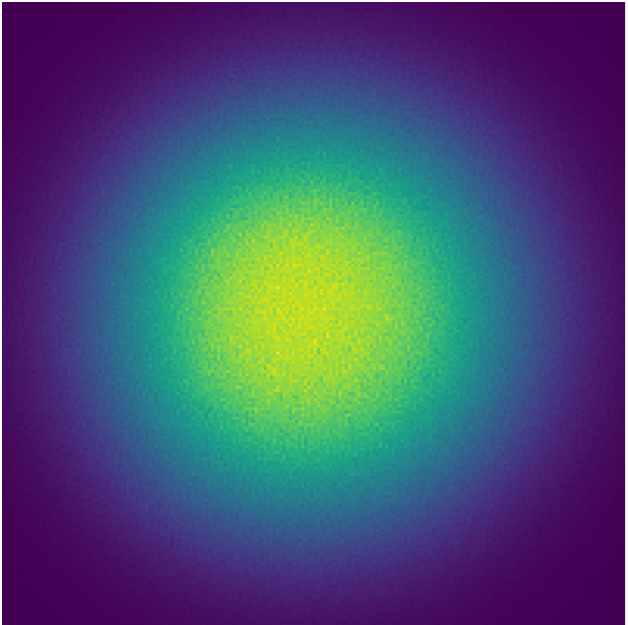
Gnomonic view
