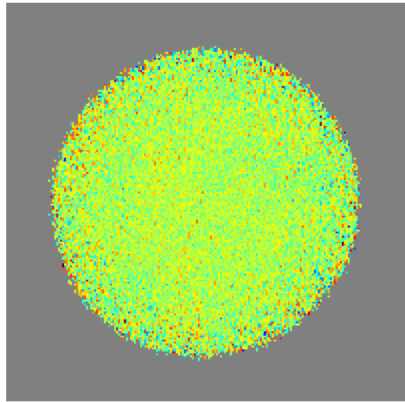
205.0 GHz - I Residual
