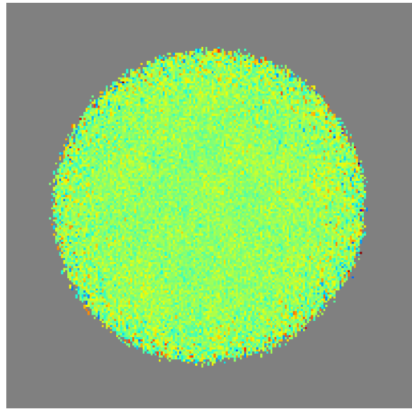
233.0 GHz - I Residual
