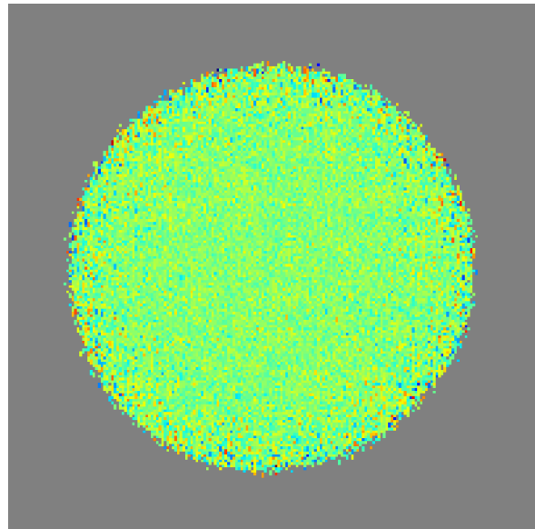
205.0 GHz - Q Residual
